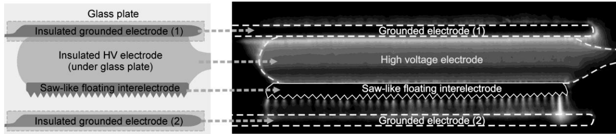
Fig. 12 Image (top view) of the discharge obtained in the double-DBD actuator with floating interelectrode. The applied sine-wave voltage was 34 \text{ kV}_{\text{pp}} , the frequency - 1.5 kHz. The camera exposure time was 0.5 s.
