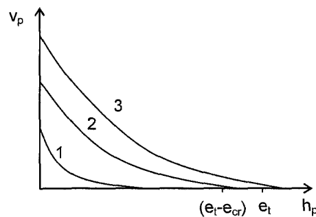
Figure 12: Relationship between the projectile velocity and the penetration depth 1 – Partial penetration in the critical domain, 2 – Partial penetration beyond the critical domain, 3 – Complete perforation
