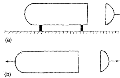
Figure 7: (a) Horizontal constrained tank; (b) Unconstrained tank [7]
