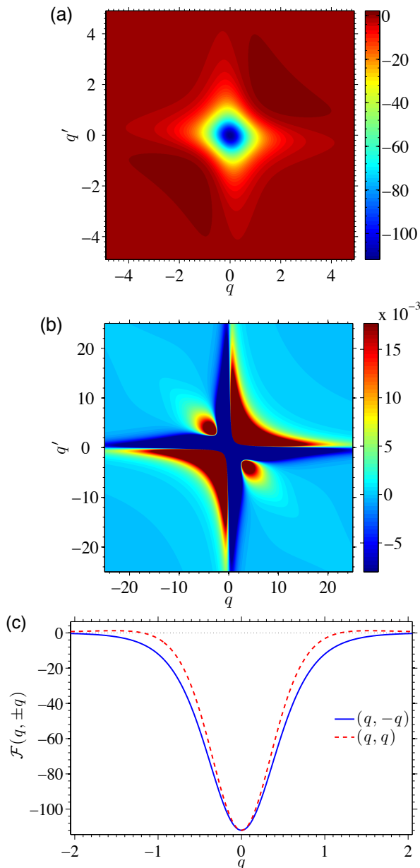
Figure 1. (Color online) (a) Dimensionless regular part of the (unnormalized) two-body momentum correlation function, \mathcal{F}(q, q') , given by Eq. (29), of a uniform 1D Bose gas in the quasicondensate regime. (b) Same as in (a), but showing the details at small correlation amplitudes (see the scale on the color bar) and in a larger window of values of (q, q') . The small negative and positive amplitudes seen here get “magnified” when the function \mathcal{F}(q, q') is normalized to \langle \hat{n}_k \rangle \langle \hat{n}_{k'} \rangle , as is done in Fig. 2. (c) Function \mathcal{F}(q, \pm q) along the diagonal ( q = q' ) and antidiagonal ( q = -q' ).
