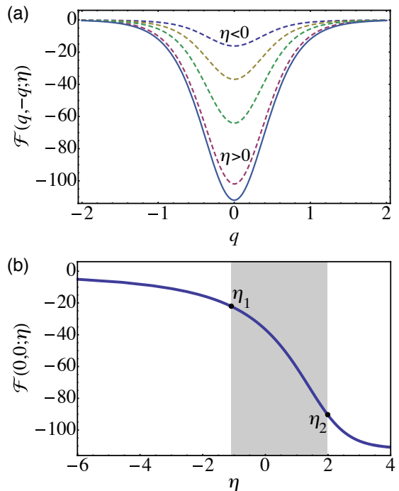
Figure 3. (Color online) (a) The antidiagonal correlation function F(q, -q; \eta) , for (from top to bottom, dashed lines) \eta = -1.87, 0, 1.12 , and 2.56 . The lowest (solid) curve is for the limiting quasicondensate regime, \mathcal{F}(q, -q) \equiv \mathcal{F}(q, -q; +\infty) , described by Eq. (29) and shown in Fig. 1 (c). (b) The minimum value of F(q, -q; \eta) as a function of \eta . The shaded area shows the crossover region between \eta_1 < \eta < \eta_2 (see text).
