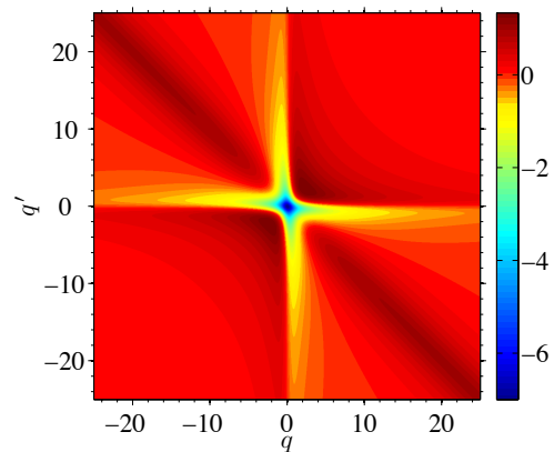
Figure 2. (Color online) Normalized regular part of the two-body correlation function f(q, q') as a function of the dimensionless momenta q = 2l_\phi k and q' = 2l_\phi k' .
