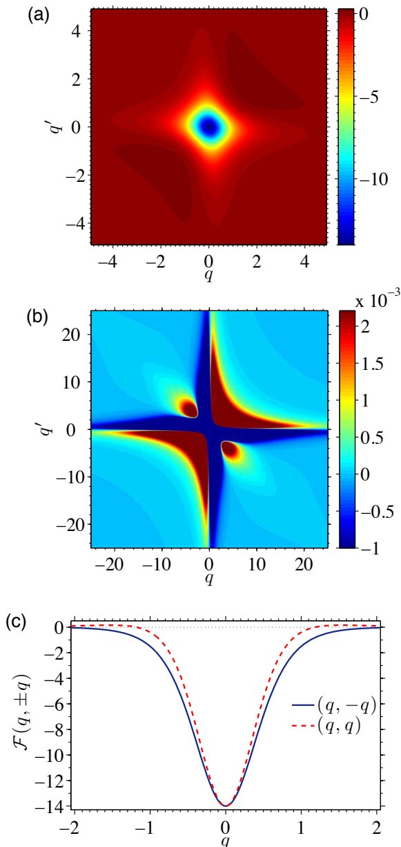
Figure 1. (Color online) (a) Dimensionless regular part of the (unnormalized) two-body momentum correlation function, \mathcal{F}(q, q') , Eq. (29), of a uniform 1D Bose gas in the condensate regime. (b) Same as in (a) but showing the details at small correlation amplitudes (see the scale on the colorbar) and in a larger window of values of (q, q') . The small negative and positive amplitudes seen here get ‘magnified’ when the function \mathcal{F}(q, q') is normalized to \langle \hat{n}_k \rangle \langle \hat{n}_{k'} \rangle as is done in Fig. 2. (c) Function \mathcal{F}(q, q') along the diagonal ( q = q' ) and anti-diagonal ( q = -q' ).
