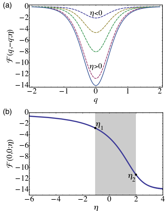
Figure 3. (a) The antidiagonal correlation function F(q, -q; \eta) , for (from top to bottom, dashed lines) \eta = -1.87, 0, 1.12, 2.56 . The lowest (solid) curve is for the limiting quasicondensate regime, \mathcal{F}(q, -q) \equiv \mathcal{F}(q, -q; +\infty) , described by Eq. (29) and shown in Fig. 1 (c). (b) The minimum value of F(q, -q; \eta) as a function of \eta . The shaded area shows the crossover region between \eta_1 < \eta < \eta_2 (see text).
