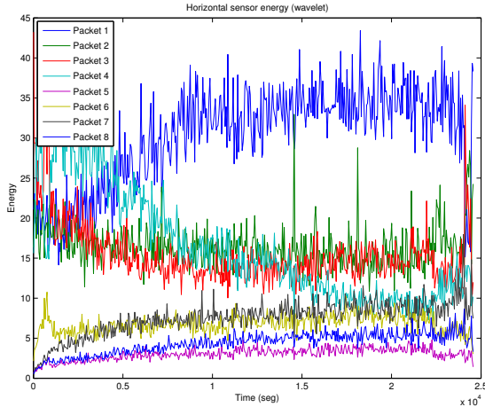
Fig. 14. Wavelet Packet Decomposition (WPD) performed on the data of the horizontal accelerometer.
