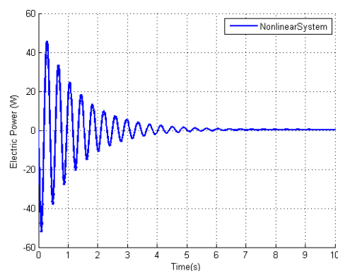
Figure 12 Response of the non linear system
