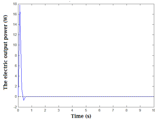
Figure 11 Response of the linear system
