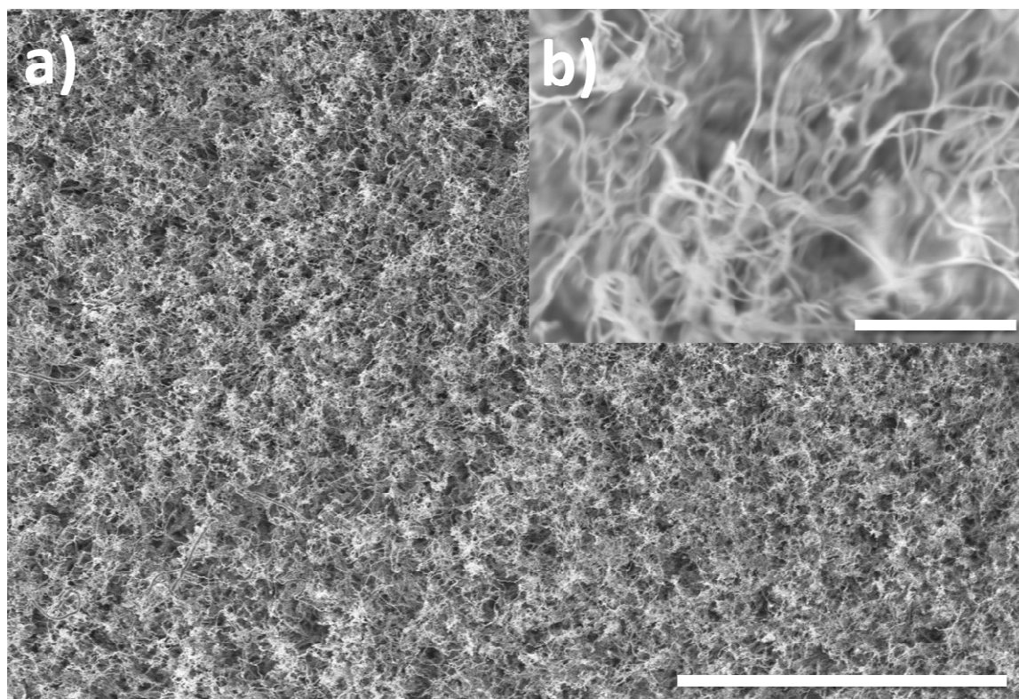
Figure 1. a) SEM image of non-organized SiO 2 NWs (scale bar = 10 μm), b) High resolution SEM image of a selected area (scale bar = 1 μm)
