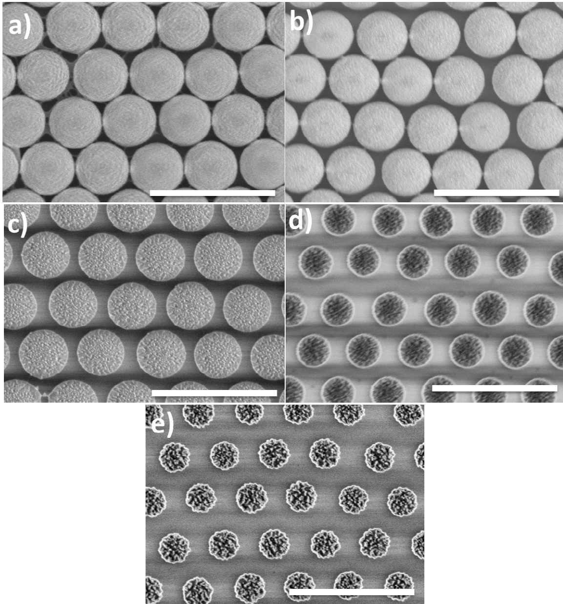
Figure 2. a) SEM images of closed-packed PS spheres arrays of 900 nm of diameter; SEM images of non-closed packed PS spheres after RIE for 1 min, 800 nm (b), 2 min, 710 nm (c), 5 min, 560 nm (d) and 7 min, 495 nm (e); (scale bars = 2 \mu\text{m} ).
