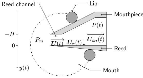
Figure 1: Schematic diagram of a single-reed mouthpiece. Presentation of variables, control parameters and choice of axis orientation. U is the flow created by the pressure imbalance P_m - P between the mouth and the bore, U_r is the flow created by the motion of the reed, U_{in} is the flow entering the instrument, y represents the position of the tip of the reed and H is the opening of the reed channel at rest.
