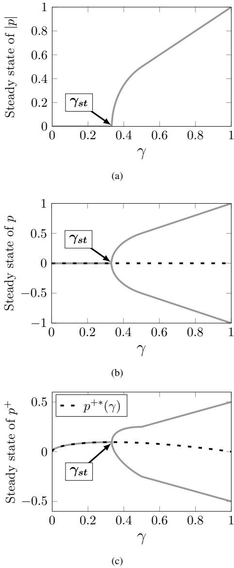
Figure 3: Graphical representation of the static bifurcation diagrams for \zeta = 0.5 . Diagrams based on variables (a) |p| , (b) p and (c) p^+ . The dashed line represents the curve of the static regime, corresponding to the fixed point p^{+*}(\gamma) of the function G_\gamma when the diagram is base on variable p^+ .
