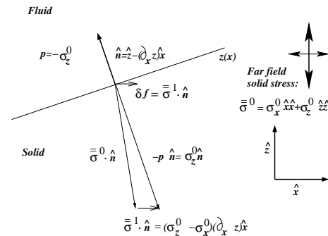
Figure 3. Local mechanical equilibrium along the fluid-solid interface (equation 8).
