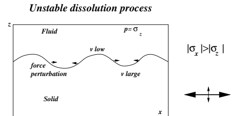
Figure 4. Surface tangential to the largest stress ( \sigma_{xx} ) axis: unstable case, Azaro-Tiller-Grinsfeld instability.
