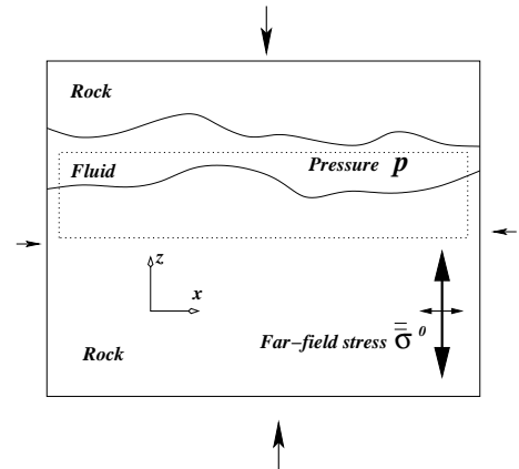
Figure 1. Initial stage of a stylolite: Trapped elongated fluid pocket.
