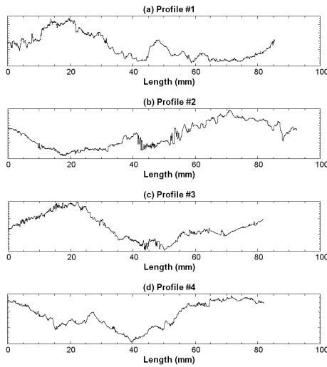
Figure 10. Functions obtained from profiles 1, 2, 3 and 4. A grey-level threshold was imposed on the pictures to isolate the stylolites. The functions were then obtained by selecting the mean limit of the pixels.
