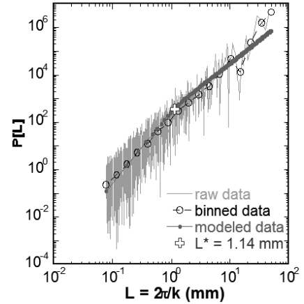
Figure 11. Fourier power spectrum of the profile 1. The raw data were binned logarithmically to run a linear-by-part fitting on the data [ Ebner et al. , 2009b]. Two different scaling regimes are observed at small and large scale with Hurst exponent around 1 and 0,5 respectively. The fit reveals a cross-over length L^* around 1.14 mm.
