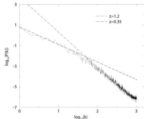
Figure 8. Average power spectrum of simulated stylolitic fronts, in bilogarithmic representation. The k -unit is 2\pi/L , with L = 4096\ell and a grain size \ell = 10\mu\text{m} . The vertical unit is arbitrary. The crossover is obtained at 2\pi/L^* .
