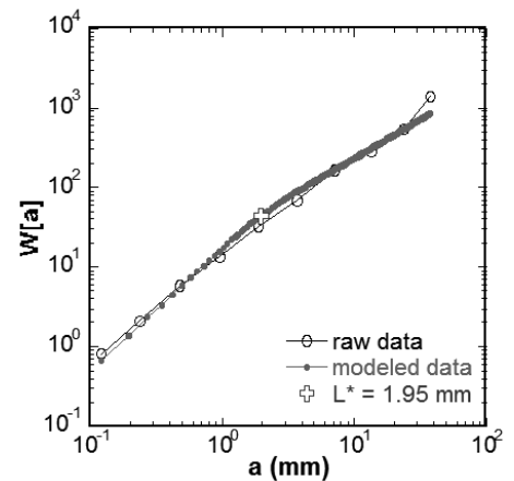
Figure 12. Averaged wavelet coefficient spectrum of the profile 1. A linear-by-part fitting were run on the data [ Ebner et al. , 2009b]. Two different scaling regimes are observed at small and large scale with Hurst exponent around 1 and 0.5 respectively. The fit reveals a cross-over length L^* around 1.95 mm. This is in good agreement with the length inferred using the Fourier power spectrum method.
