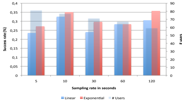
Figure 3: Success rate of the linear/exponential weighted votes.
