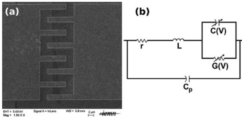
Figure 1. Photograph of an InterDigitated Capacitance (IDC) on a micron scale (a). RLC equivalent circuit of the IDC (b).
