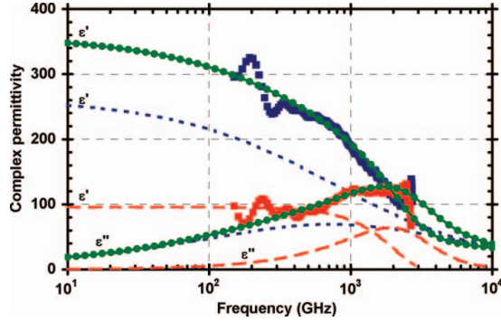
Figure 4. Complex dielectric dispersion of the BST thin film measured (square) and retrieved (circle) with dipole polarization part (dotted lines) and ionic polarization part (dashed lines) (Figure available in color online).
