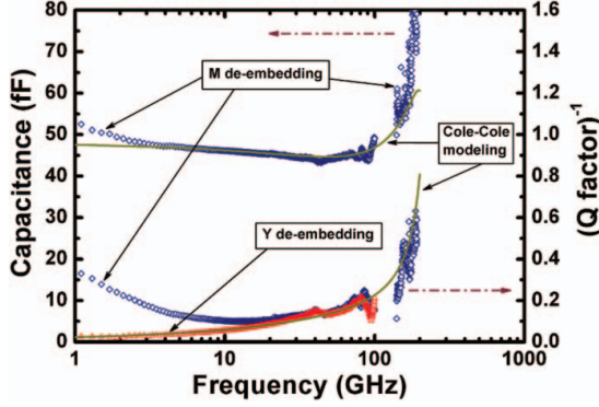
Figure 2. Frequency dependences of the apparent capacitance and of the inverse of the quality factor of the IDC (Figure available in color online).
