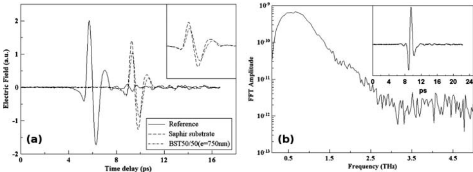
Figure 3. Reference, sapphire, and BST onto sapphire transmitted electric field in time domain (a). FFT amplitude of the THz reference pulse (b).
