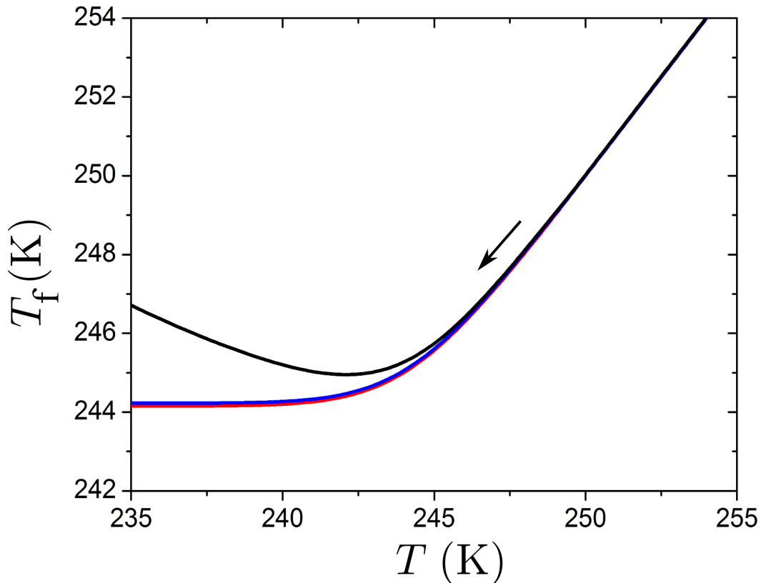
Figure 11: Fictive temperatures as a function of temperature during cooling at a temperature rate of -0.5 K/min at constant pressure of 0.1 MPa. The red one, which comes from the classical definition of the fictive temperature, is issued from integration of the corresponding normalized heat capacity data. The blue one is issued from the Eq. (28). The black one is inferred from calculation of Tropin and co-workers with an approximate value of the affinity (see Eq. (50) of Ref. [22]).
