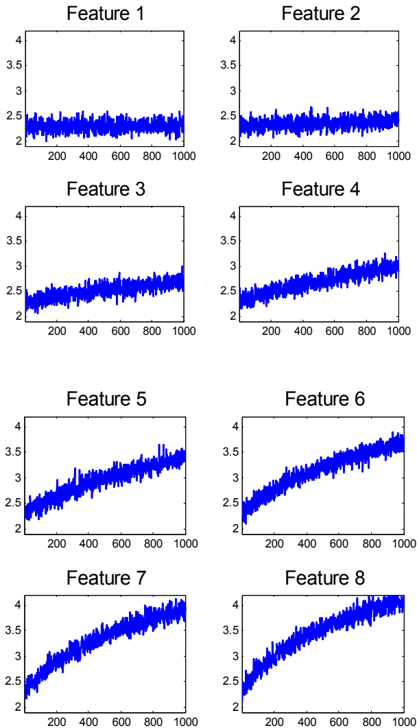
Figure 5. Simulated Features.
