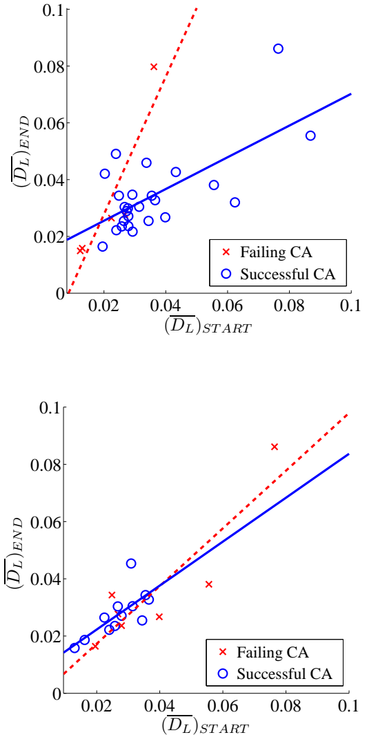
Fig. 2: Scatter plot of \overline{D}_L END as a function of \overline{D}_L START and data regression lines associated with each category (successful CA: O, continuous line; failing CA: ×, dotted line.). (Top) Short-term success; (Bottom) Long-term success.
