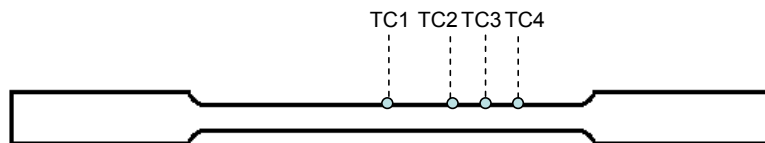
Figure 3 – Geometry of the reduced central section cylindrical sample used in the Gleeble simulation experiment (TC1, TC2, TC3 and TC4 refer to the positions of the thermocouples).
