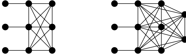
Figure 3: The urchins W(3,3) and W(3,5)
