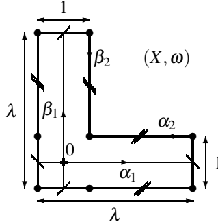
FIGURE 2. An L-shaped translation surface with an order 4 automorphism
