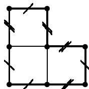
FIGURE 1. The L-shaped translation surface tiled by three squares
