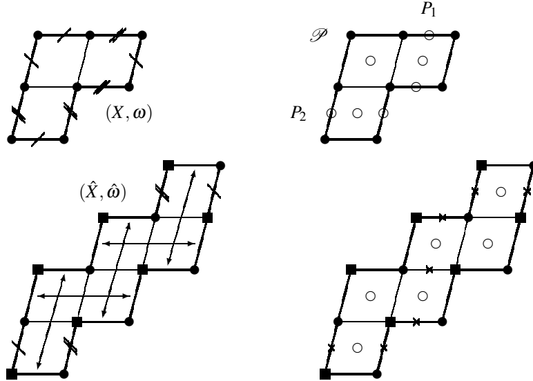
FIGURE 4. Double cover: identifications and Weierstrass points
