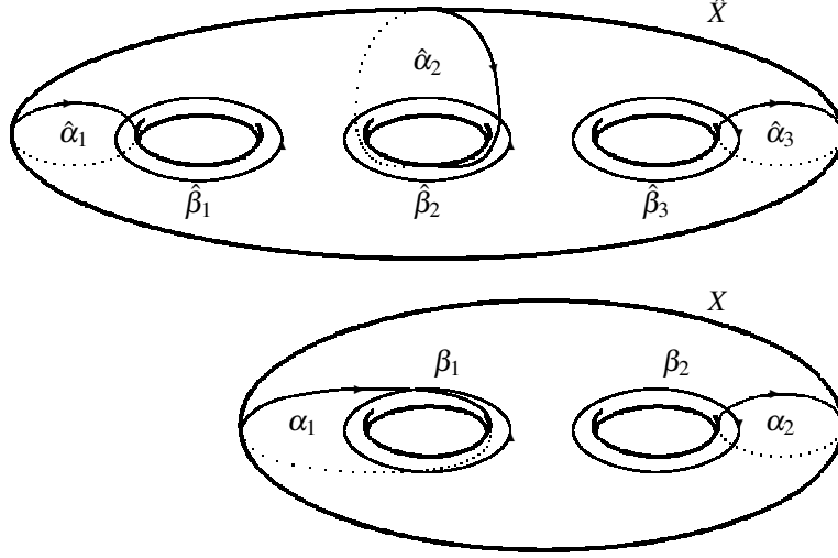
FIGURE 5. Homology bases for X and \hat{X}
