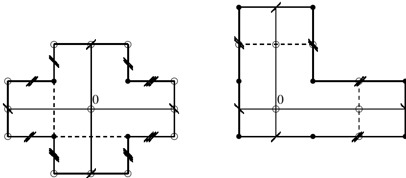
FIGURE 3. A L-shaped translation surface defines a real M-curve
