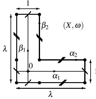
FIGURE 2. An L-shaped translation surface with an order 4 automorphism
