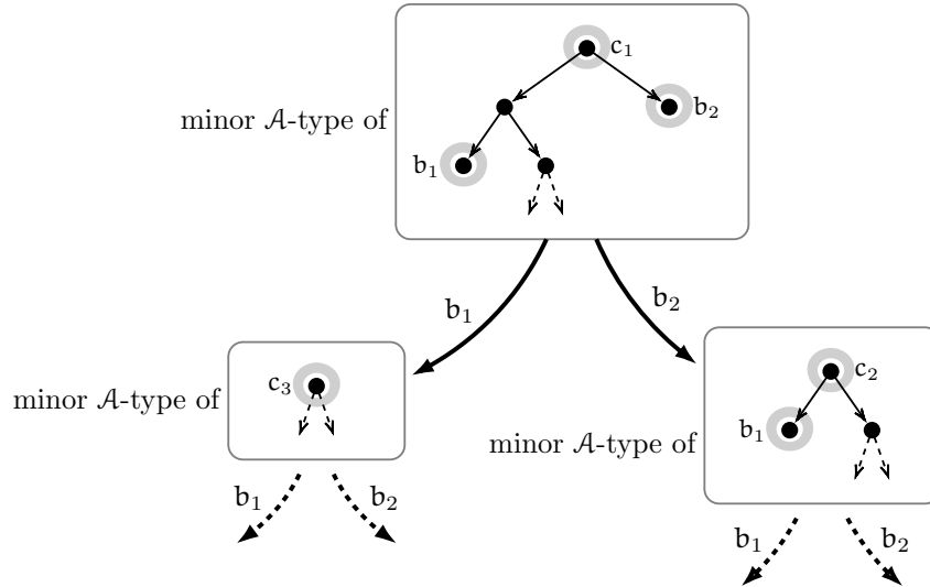
Fig. 3.3. An example of retraction
