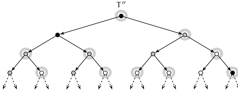
Fig. 3.6. Another distorted tree from Example 3
