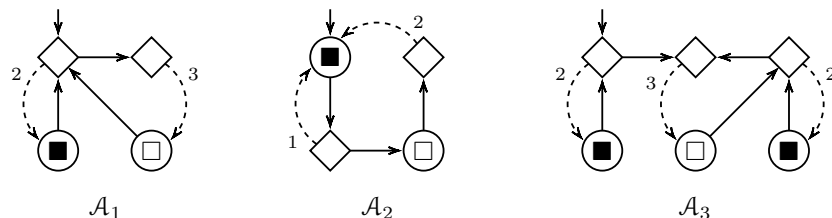
Fig. 2.8. State-optimal and complexity optimal NCSSA
