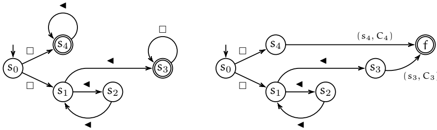
Fig. 2.13. Equivalence of UPA does not transfer to their prefix automata
