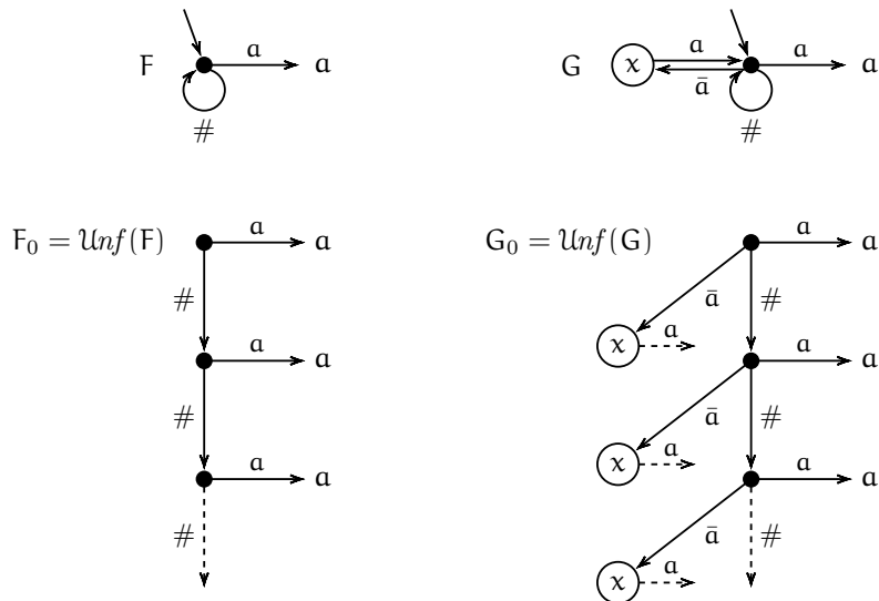
Fig. 3.16. Marked factors for the two-way unfolding of the semi-infinite line
