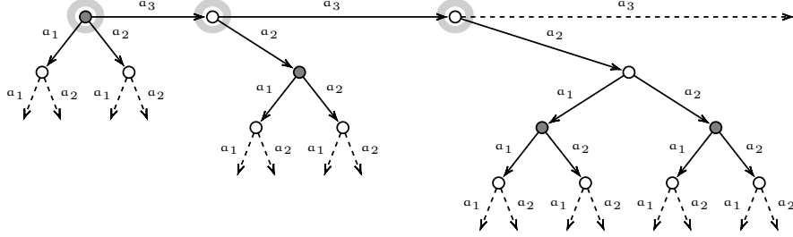
Fig. 3.23. The ternary colored tree embedding TULS^{\neq, L_0}
