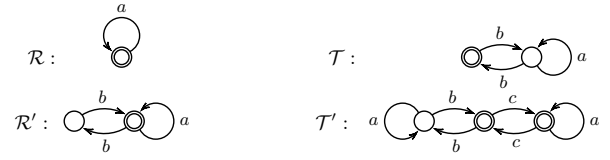
Figure 1: Some non-deterministic Büchi automata.
