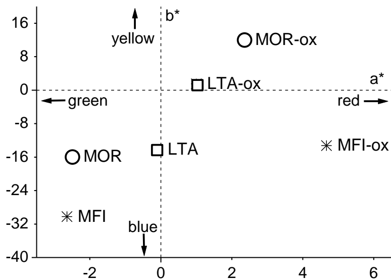
Fig. 3 – Projection on the a*b* space of 3 indigo@zeolite samples before and after oxidising test (10 minutes in concentrated HNO 3 , 14mol/l). LTA = indigo@LTA zeolite; MOR = indigo@mordenite; MFI = indigo@silicalite. Suffix -ox is added to distinguish samples after the oxidising test.
