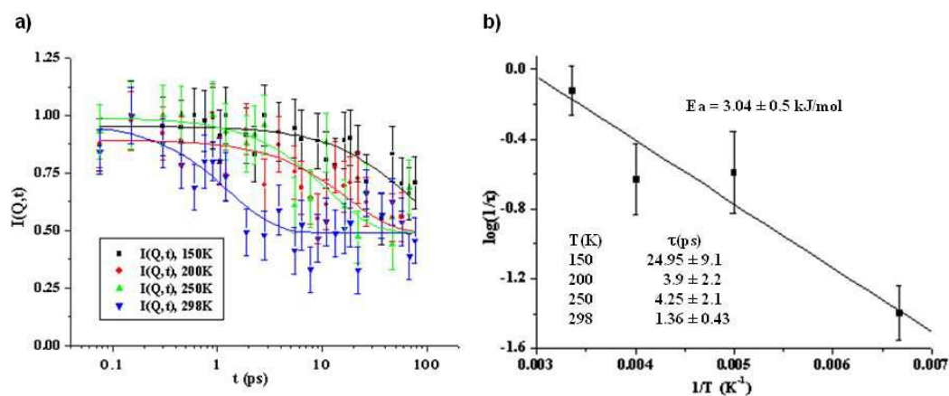
Fig. 2. a) Intermediate scattering function obtained for dmpNA encapsulated in silicalite at: 150 \text{ K} , 200 \text{ K} , 250 \text{ K} and 298 \text{ K} , for Q = 0.9 \text{ \AA}^{-1} . b) Characteristic frequency ' 1/\tau ' versus temperature ' T '. The solid line is the calculated Arrhenius law from a least squares fitting.
