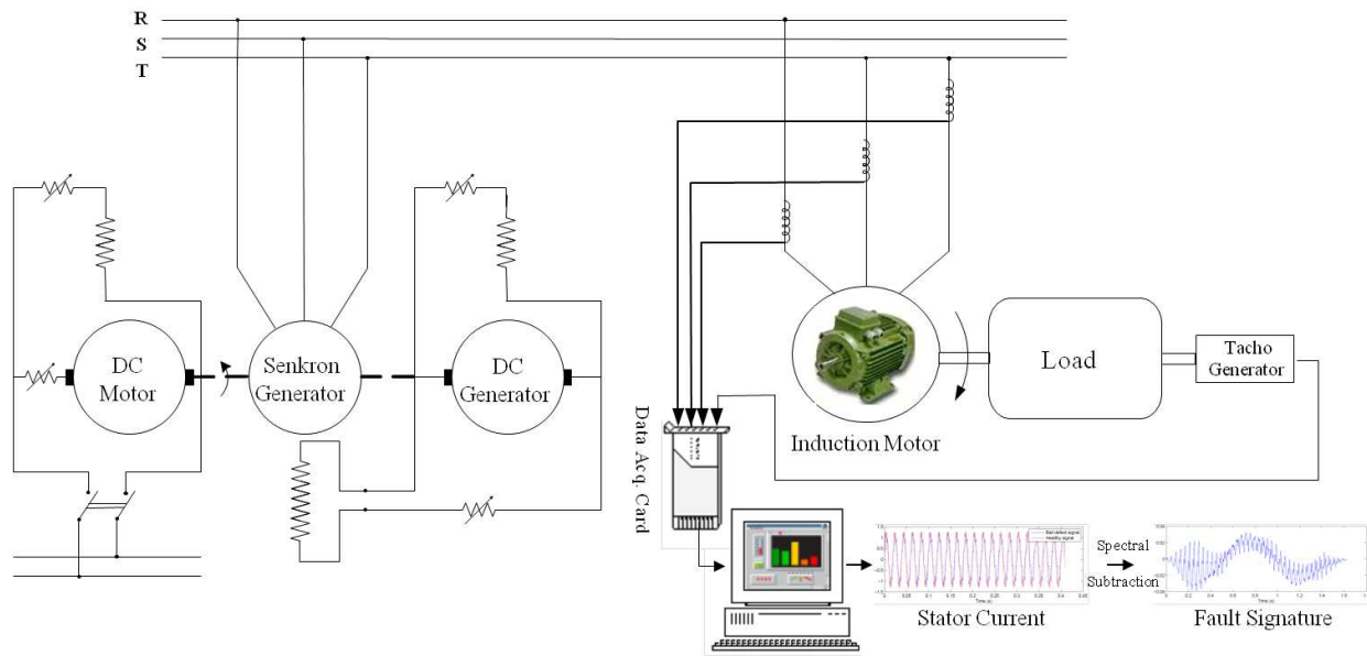
Fig. 5: Scheme of the experimental set up.
