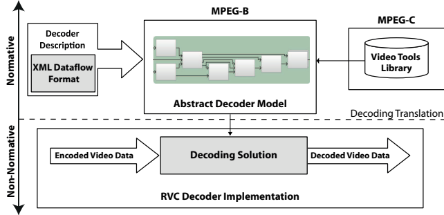
Figure 2: A typical use of the MPEG RVC Framework.
