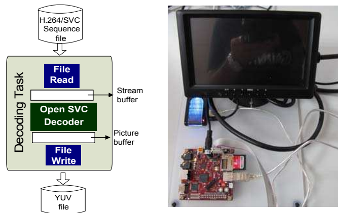
a) Test-bench used to profile the OSD in real time. b) Prototyping system based on a commercial processor [5].
