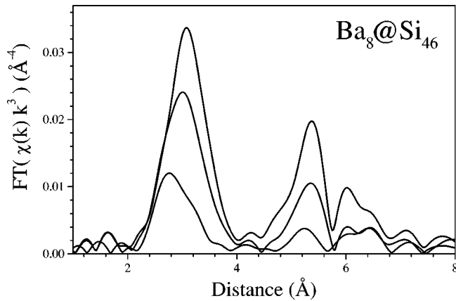
FIG. 3. Fourier transform of the EXAFS signal at T=20, 100, and 300 K. The signal amplitude decreases with the temperature.
