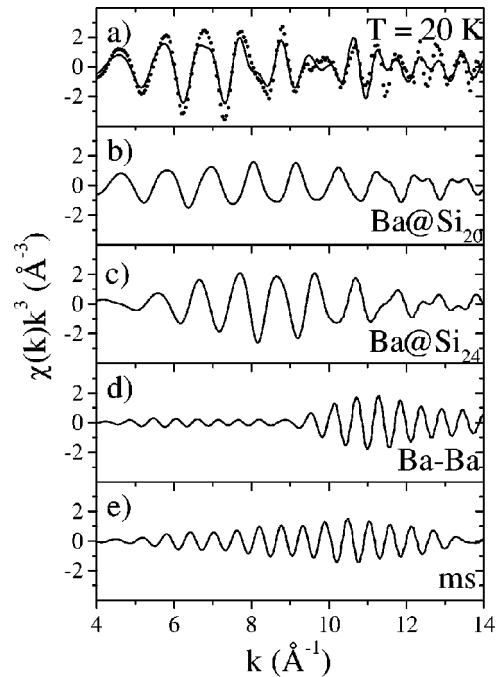
FIG. 4. (a) Experimental EXAFS oscillations at 20 K (dots) and best fit (continuous line) obtained with the Ba atoms placed at the center of the cages. The following panels show a decomposition of the signal that includes: (b) single-scattering paths having as origin the \text{Ba@Si}_{20} ; (c) single-scattering paths having as origin the \text{Ba@Si}_{24} ; (d) Ba-Ba single-scattering paths; (e) all multiple-scattering paths.
