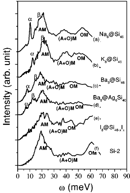
FIG. 1. Inelastic-scattering data determined at 300 K of various silicon clathrates (a)–(e) and pure silicon (f). \alpha and \beta design the low-frequency molecular modes (mmf) corresponding to the rattling of the entrapped atoms in the cages. AM , OM , and (A+O)M stand, respectively, for acoustic modes, optic ones, and the mixed contribution of the two.
