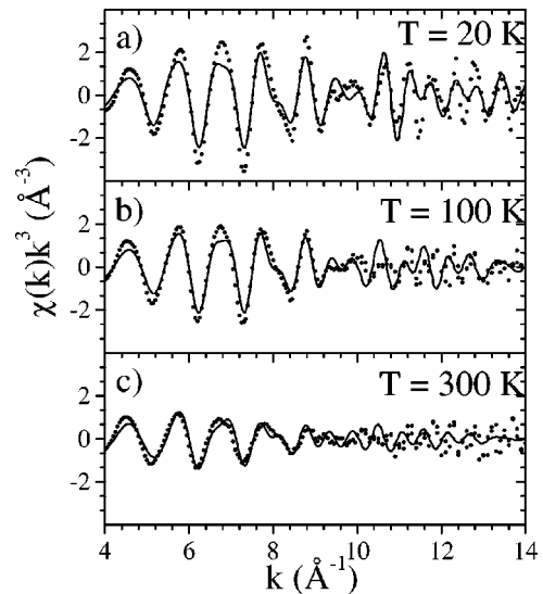
FIG. 2. Dots: Experimental EXAFS oscillations of Ba_8Si_{46} at the Ba K -edge at T=20, 100, and 300 K. The signal has been multiplied by k^3 . Lines: corresponding fit of the data obtained with the Ba atoms placed at the center of the cages (see text for details). We note that at 300 K, the noise level dominates the signal for k values higher than 10 \text{ \AA}^{-1} .
