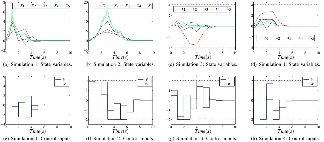
Fig. 2. States and control variables of the chained system. Simulation 1: without constraints. Simulation 2: with control constraints. Simulations 3 and 4: with state and control constraints.
