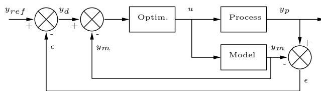
Fig. 1. Control Structure
