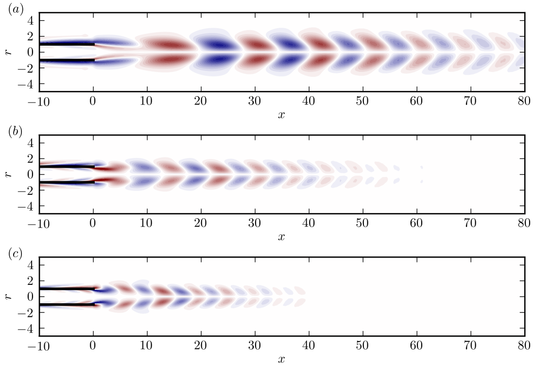
Figure 9: Real part of the vorticity fields of typical eigenmodes, labeled in figure 8a, in an isothermal jet at Re = 100 , Ma = 0.75 and Pr = 1 . (a) \omega = 0.26 - 0.026i . (b) \omega = 0.50 - 0.040i . (c) \omega = 0.71 - 0.047i .
