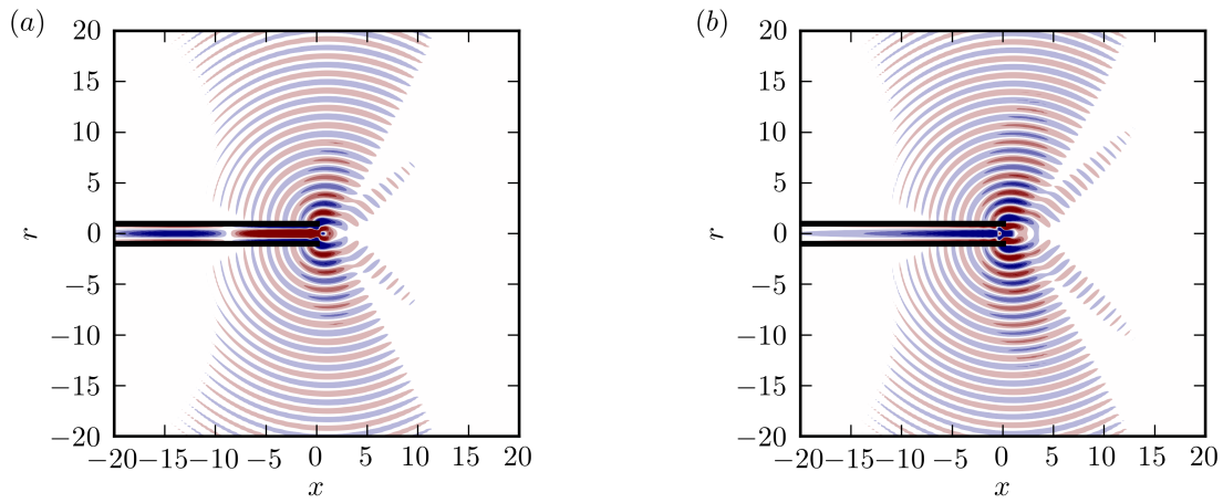
Figure 10: Real part of the dilatation fields of typical eigenmodes, labeled in figure 8a, in an isothermal jet at Re = 100 , Ma = 0.75 and Pr = 1 . (a) \omega = 4.9 - 0.17i . (b) \omega = 5.1 - 0.18i .
