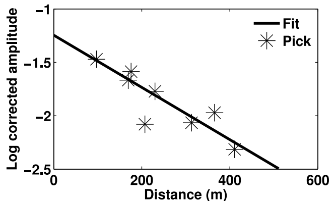
Figure 7. The natural logarithm of the geometrically corrected maximum Rayleigh wave amplitude pick as a function of epicentral distance for a single type A event. The remaining decay in the corrected amplitudes is attributed to the seismic quality factor Q . In this example we estimate Q \approx 35 .
