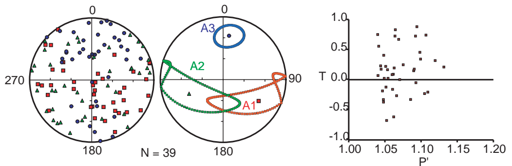
Figure 4: A-ARM fabrics, equal-area diagrams, lower hemisphere projections in geographical frame and Jelinek diagrams. a) Samples from lava flows yielding a normal fabric. b) Samples from lava flows yielding an abnormal fabric. In equal-area projections, squares are maximum ARM ( A_1 axes), triangles are intermediate ARM ( A_2 axes), and circles are minimum ARM ( A_3 axes). Confidence ellipses were calculated by means of Jelinek's statistics.
