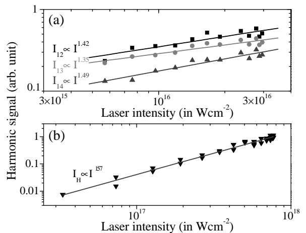
FIG. 41: (a) Intensity dependence of the harmonic signal for three different CWE harmonics, produced with the LUCA laser. The laser intensity was varied using an attenuator (combination of a half wave-plate and two polarizers). (b) Intensity dependence of the spatially and spectrally-integrated harmonic signal, measured experimentally in the non-relativistic regime with the UHI10 laser. In these case the different points have been obtained by simply varying the laser polarization (from pure p to pure s ). The harmonic beam goes through a 200 nm thick Indium filter which mainly transmits orders 10 to 15.
