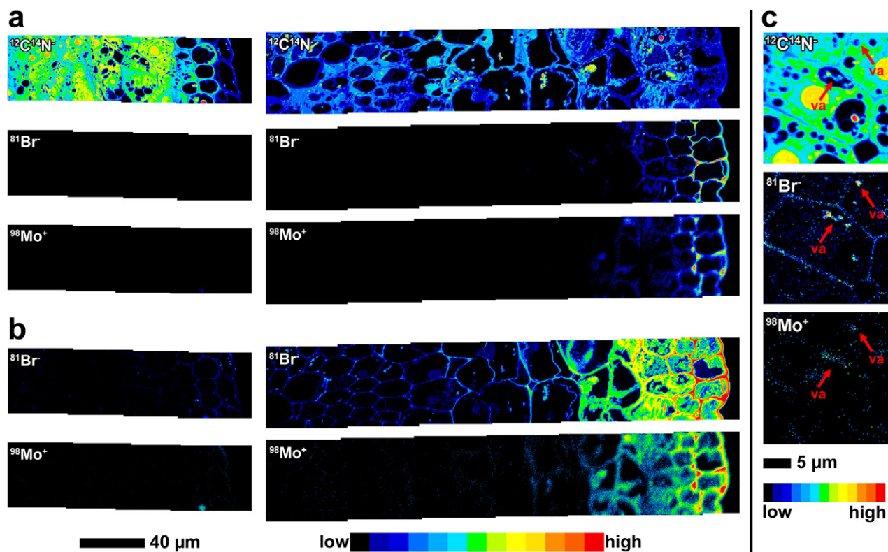
Fig. 5. NanoSIMS maps of ^{12}\text{C}^{14}\text{N}^- , ^{81}\text{Br}^- and ^{98}\text{Mo}^+ secondary ions in whole (a and b) or cortex (c) root cross sections of plants treated with a water-sorbing cluster suspension (left column in figures a and b, and figure c) or ethanol-sorbing cluster solution (right column in figures a and b), both at 1 mM, with (a and c) decimal and (b) logarithmic color scales. Analyzed samples are transversal sections of the roots, made few millimeters from the apex after chemical fixation, resin embedding and ultramicrotome sectioning. For every strip (a and b) the external part of the root is on the right side and the center of the root is on the left side of the strip. Arrows (c) indicate some cluster aggregates in vacuoles (va). (For interpretation of the references to color in this artwork, the reader is referred to the web version of the article.)
