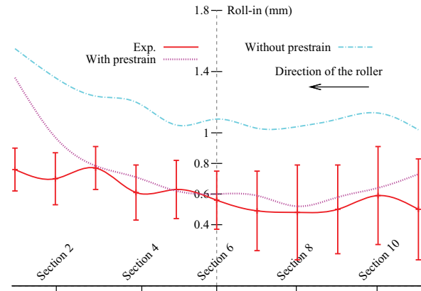
Fig. 14. Influence of the mechanical fields from the biaxial expansion and flanging steps on the prediction of roll-in during hemming. Simulations are performed with Hill48-Mixed model.
