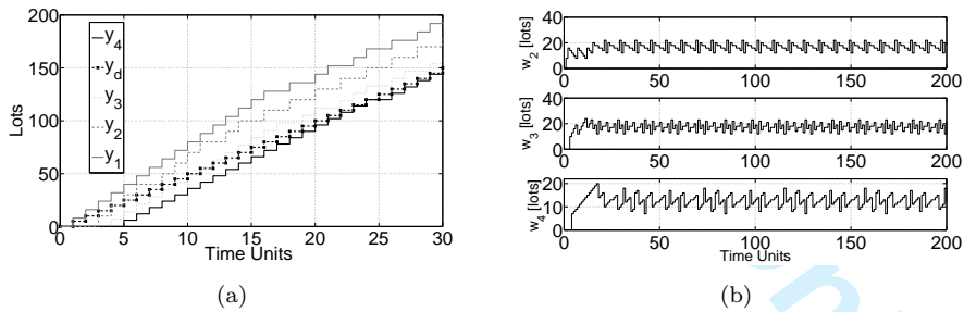
Figure 6. Outputs y_j(k) vs. Demand y_d(k) (a) and Buffer Content w_j(k) (b), with v_d = 5 .
