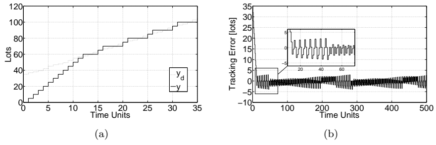
Figure 4. Demand vs Output (a) and Tracking Error (b), with y_{d0} = 35, v_d = 2 and \varphi(k) = \sin(5k) .
