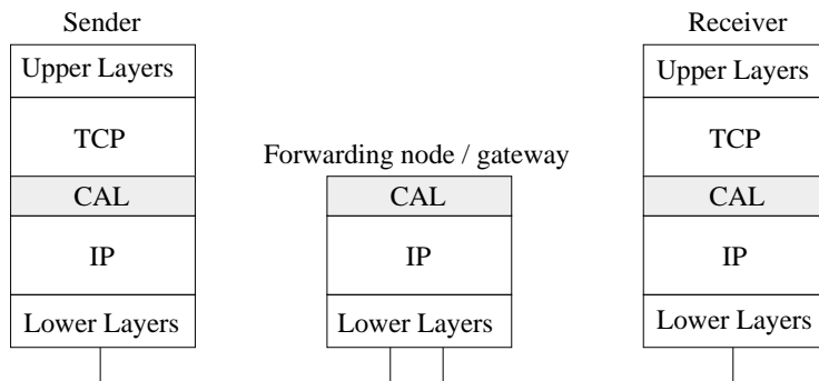
Figure 2. The proposed IP-ERN architecture.
