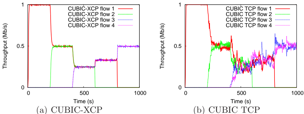
Figure 14. Intra-fairness
