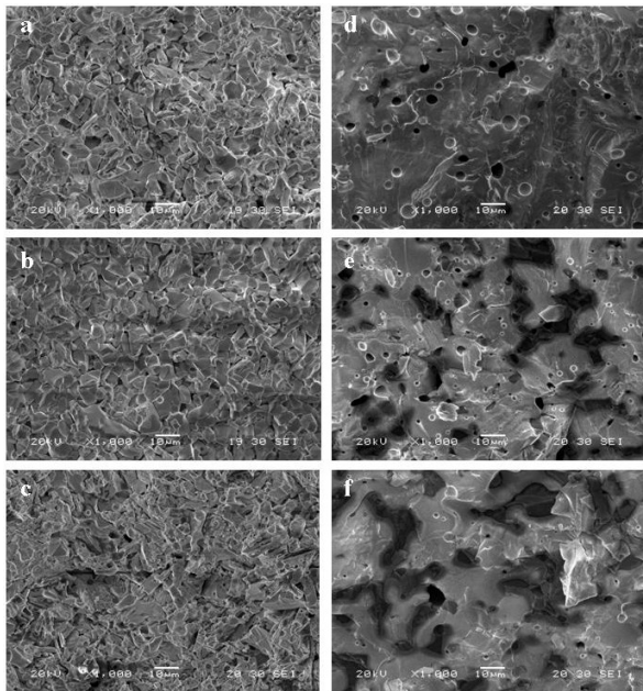
Figure 6: SEM images for \text{Hf}_{1-x}\text{Mn}_x\text{O}_{2-\delta} with different Mn content (a) x = 0.05 ; (b) x = 0.10 ; (c) x = 0.20 ; (d) x = 0.30 ; (e) x = 0.40 ; (f) x = 0.50 .
