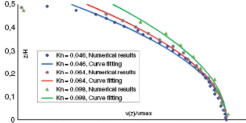
Fig. 3 Velocity profiles for the upper half of the channel obtained by MD simulation (marker line) and fitted by analytical formula (solid line). In the figure, the acceleration \gamma_x is kept constant at 0.012 \text{ \AA/ps}^2 while the Knudsen number is varied. The vertical and horizontal axis represent normalized coordinate, z/H and velocity, v(z)/v_{\max} , along the flow direction. The velocity v_{\max} is the maximal velocity found in the middle of the channel
