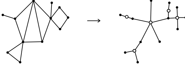
Figure 1: The block-decomposition of a connected planar graph. In the associated tree (incidences between 2-connected blocks and vertices) there is a white vertex for each block.
