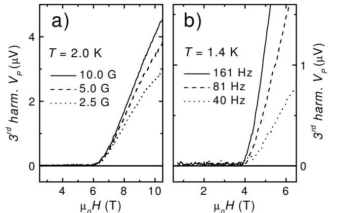
FIG. 6: Third harmonic response measured after averaging over the oscillations in a resistive coil for different modulation amplitudes (a) and modulation frequencies (b). The critical field values obtained at a given temperature are independent on modulation frequency and amplitude.
