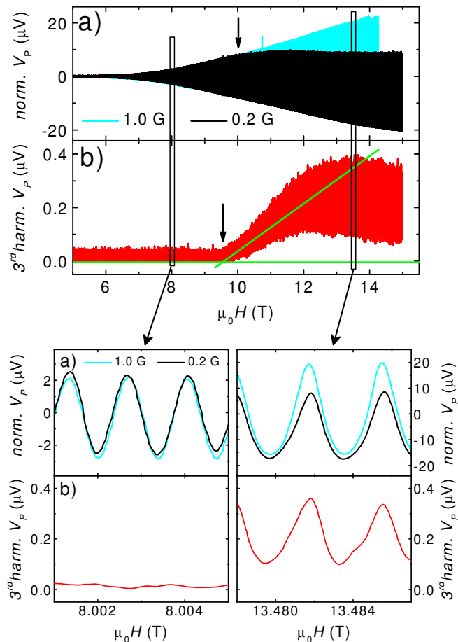
FIG. 3: (Color online) (a) Pickup voltage normalized on the modulation level for low and high modulation level. Up to about 10 T the response is linear with respect to the modulation level. (b) Third harmonic of the pickup voltage measured at 0.2 G modulation amplitude showing that starting from 9.5 T the harmonic content in the response increases steeply. Lower part of the figure shows respective zooms. Both data measured at 2.7 K.
