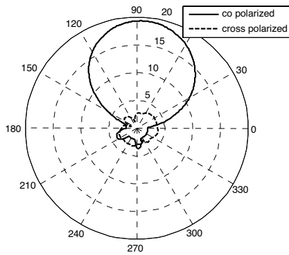
Figure 3. Co & cross polarized patterns at 900 MHz.
