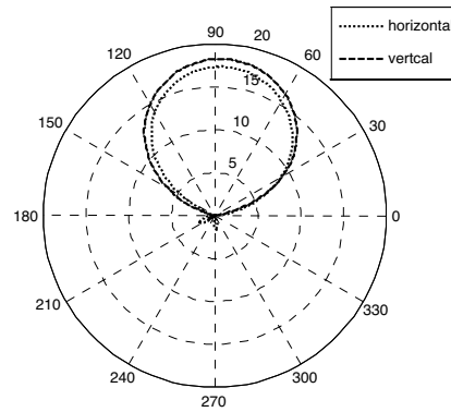
Figure 4. Patterns at 900 MHz with transmitter in horizontal and vertical directions.
