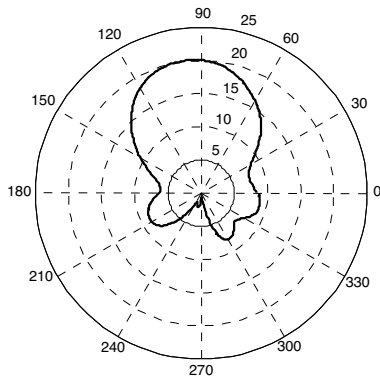
Figure 7. Measured pattern in y - z plane and 900 MHz.
