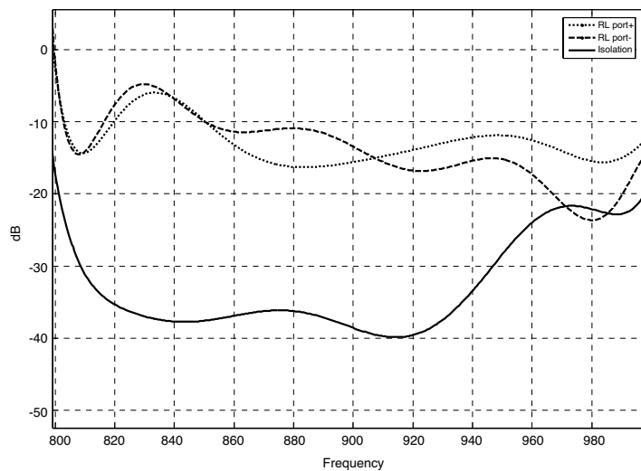
Figure 9. Measured RL and isolation between positive and negative ports at 900 MHz.
