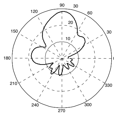
Figure 8. Measured pattern in y - z plane and 1800 MHz.
