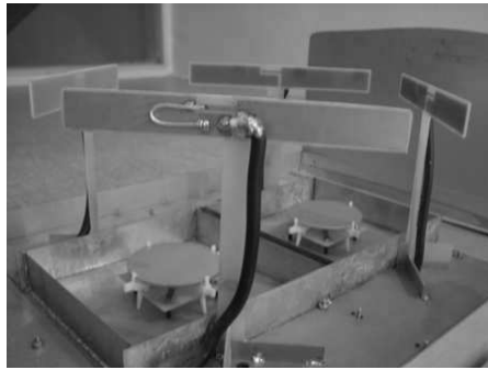
Figure 2. Dual polarized patch and dipoles structure.
