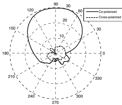
Figure 5. Co & cross polarized patterns at 1800 MHz.
