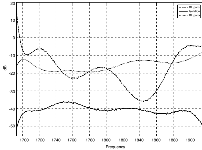
Figure 10. Measured RL and isolation between positive and negative ports at 1800 MHz.
