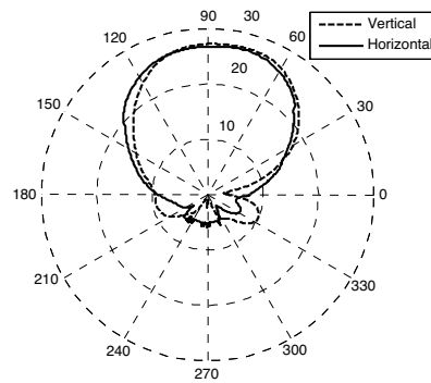
Figure 6. Patterns at 1800 MHz with transmitter in horizontal and vertical directions.
