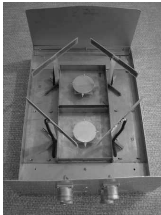
Figure 1. Proposed antenna structure.
