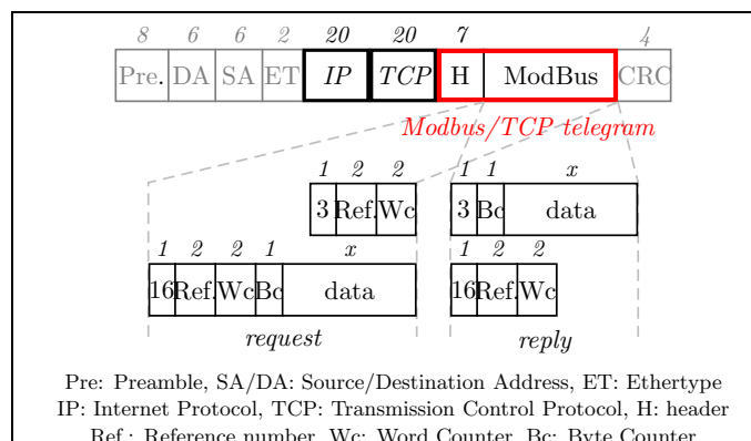
Figure 8: General Modbus/TCP frame and function specific Modbus application frame ( field lengths are given in bytes )
