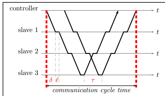
Figure 2: EtherCAT space-time diagram
