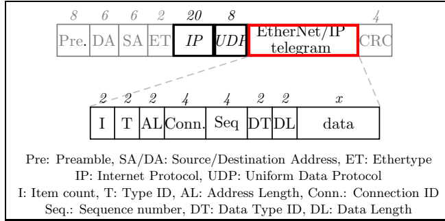
Figure 12: EtherNet/IP I/O messaging frame ( field lengths are given in bytes )
