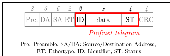
Figure 7: Profinet IRT frame ( field lengths are given in bytes )
