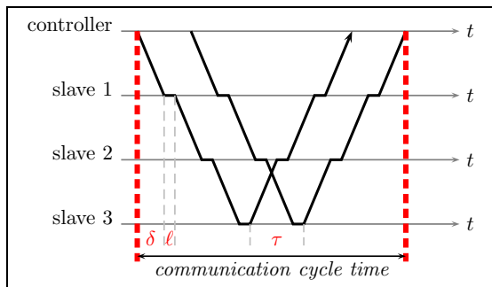
Figure 2: EtherCAT space-time diagram
