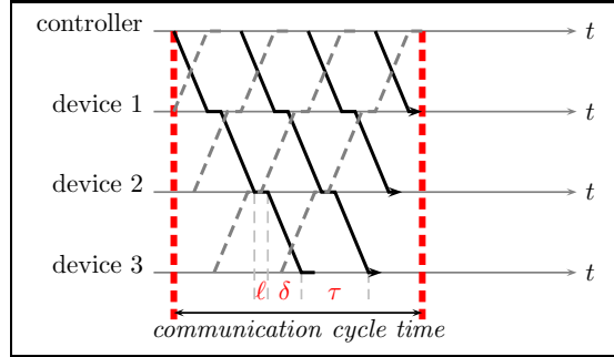
Figure 6: Profinet IRT space-time diagram with slipstreaming effect
