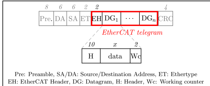
Figure 4: EtherCAT frame ( field lengths are given in bytes )
