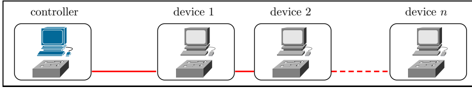
Figure 5: Profinet line topology
