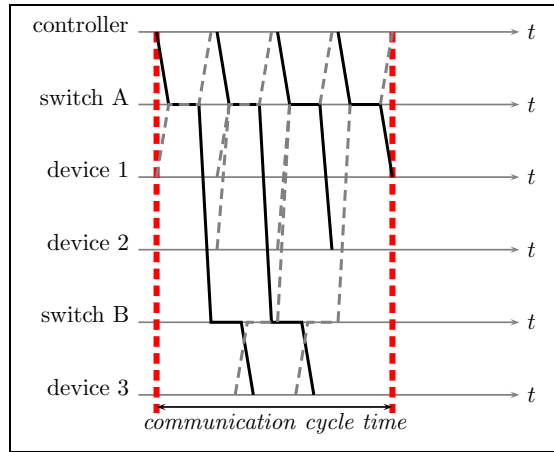
Figure 11: EtherNet/IP space-time diagram for 4-ports switches
