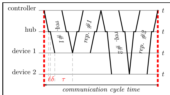
Figure 9: Modbus/TCP space-time diagram
