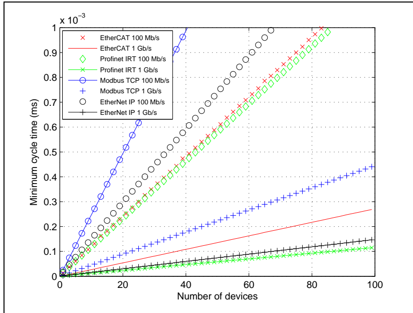
Figure 13: Minimum cycle time as a function of the number of devices with a constant payload of 100 bytes per device and two bit rates of 100 Mb/s and 1 Gb/s
