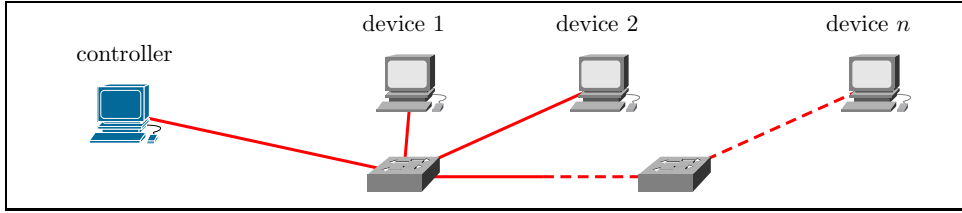
Figure 10: EtherNet/IP switched linear topology
