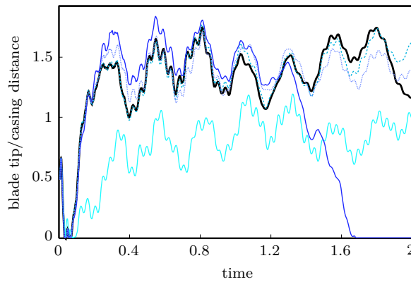
(b) Locked motion, blade 9
