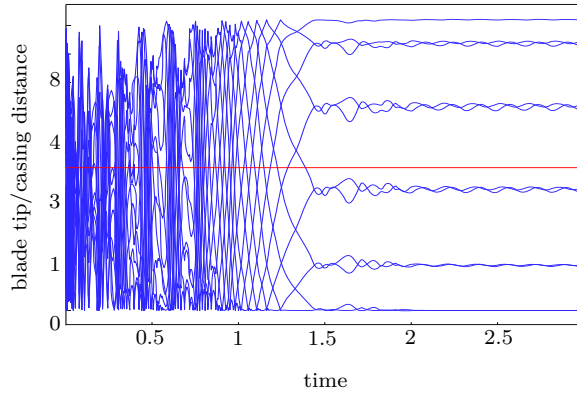
(c) Locked motion: \Omega = 0.55 , n_d = 2
