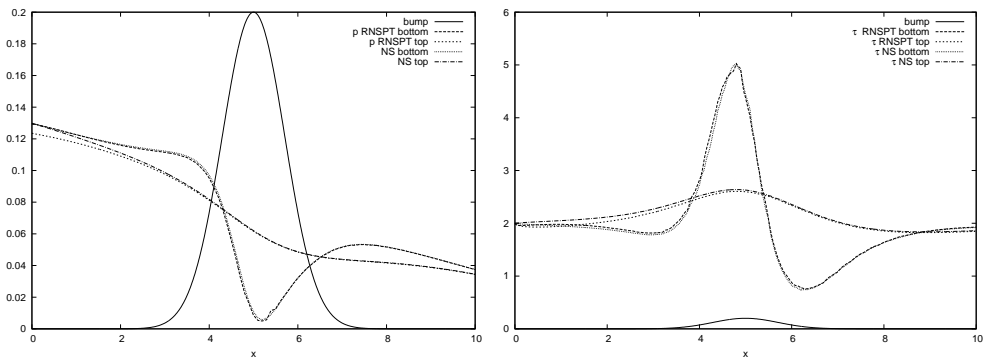
Figure 8: Comparing NS and RNSP with Transverse effects. Flat upper wall, and bumpy lower wall. Observe the upstream influence of the Skin friction and of the pressure.
