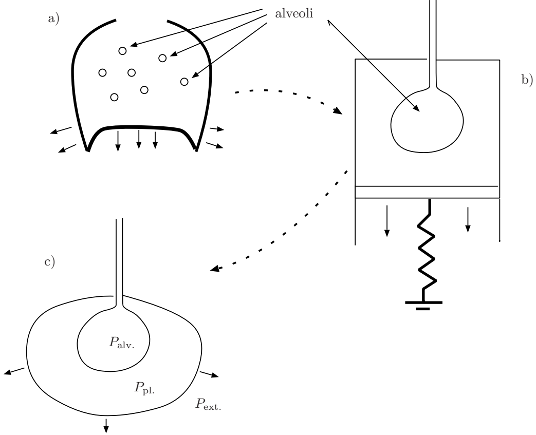
Figure 2: Double-balloon model
