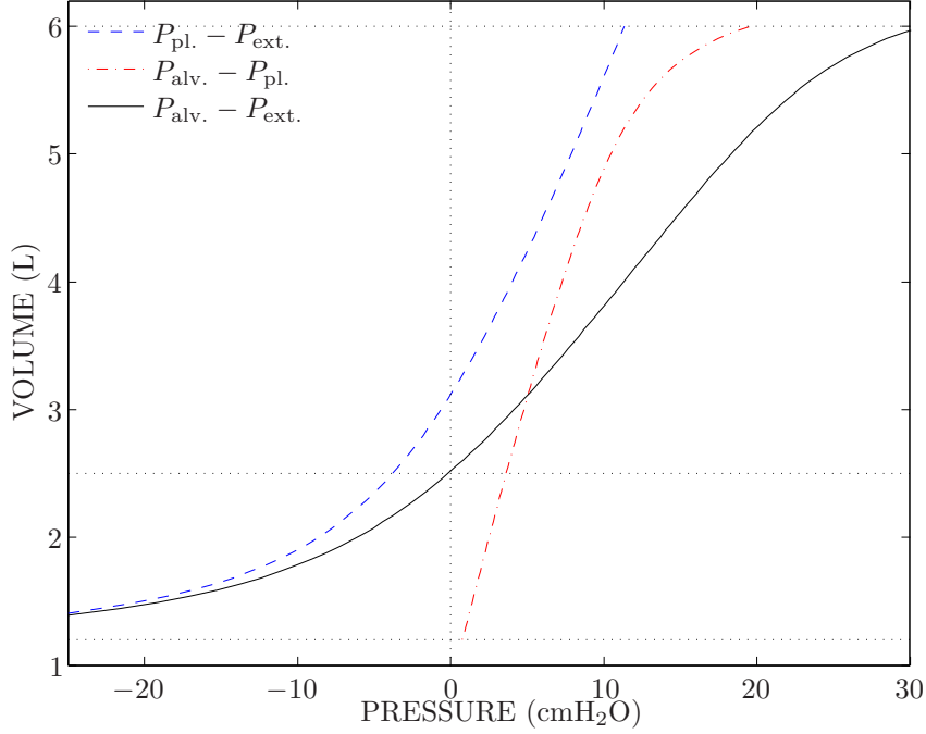
Figure 3: Elastic behavior of the lung: relation between the lung volume V and the difference of pressure \Delta P (from [1]) for typical values of V_{RV} = 1.2\text{ L} , V_{FRC} = 2.5\text{ L} and V_{TLC} = 6\text{ L} .
