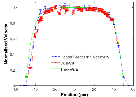
Figure 2: Normalized profiles of maximal velocity measured in a rectangular PDMS channel ( 100\mu\text{m} \times 20\mu\text{m} ), using OFI (blue curve) and DS (red curve).
