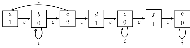
Fig. 1. A (bounded) parity game with costs.
