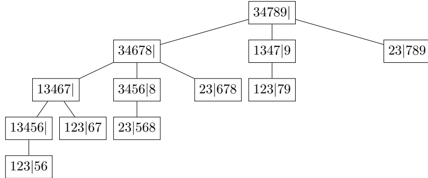
FIGURE 5. The negative greedy flip tree \mathcal{N}(\bar{Q}, \bar{\rho}) on the subword complex of Example 2.2. Each facet I is denoted as the concatenation of its elements. The symbol | separates the elements smaller or equal to n(I) from those which are strictly larger than n(I) .
