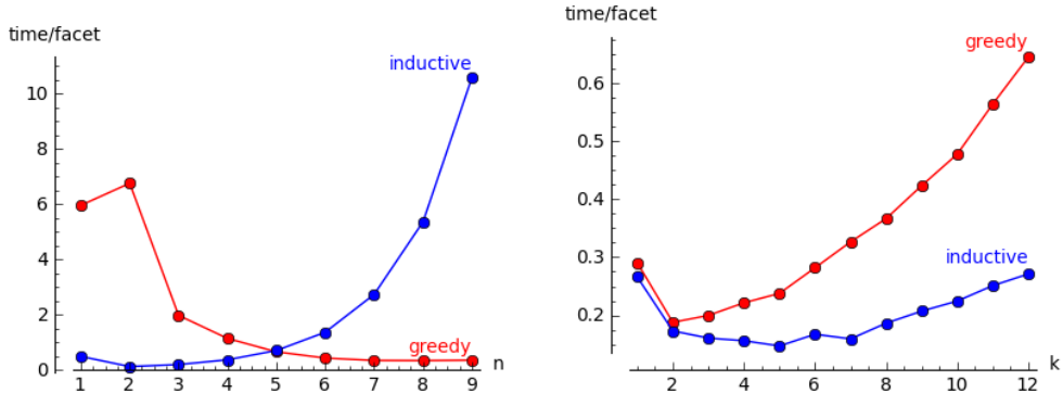
FIGURE 7. Comparison of the running times of the inductive algorithm and the greedy flip algorithm to generate the k -cluster complex of type A_n . On the left, k is fixed to 1 while n increases; on the right, n is fixed to 3 while k increases. The time is presented in millisecond per facet.
