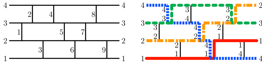
FIGURE 1. The network \mathcal{N}_{\bar{Q}} (left) and the pseudoline arrangement \Lambda_I for the facet \bar{I} = \{1, 3, 4, 7, 9\} of \mathcal{SC}(\bar{Q}, \bar{\rho}) (right).
