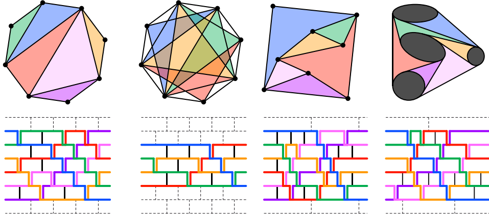
FIGURE 2. Primitive sorting networks are combinatorial models for certain families of geometric graphs.
