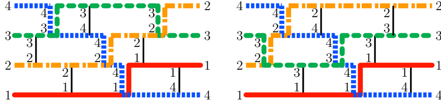
FIGURE 4. The flip between the adjacent facets \bar{I} = \{1, 3, 4, 7, 9\} and \bar{J} = \{3, 4, 7, 8, 9\} of \mathcal{SC}(\bar{Q}, \bar{\rho}) , illustrated on the network \mathcal{N}_{\bar{Q}} .
