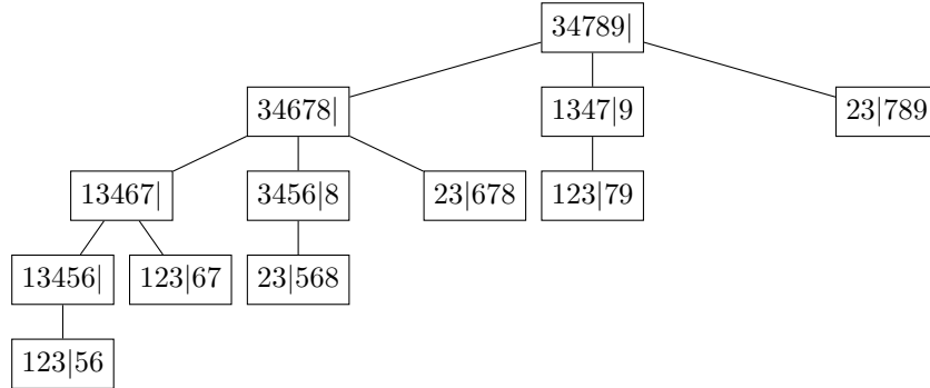
FIGURE 5. The negative greedy flip tree \mathcal{N}(\bar{Q}, \bar{\rho}) on the subword complex of Example 2.2. Each facet I is denoted as the concatenation of its elements. The symbol | separates the elements smaller or equal to n(I) from those which are strictly larger than n(I) .
