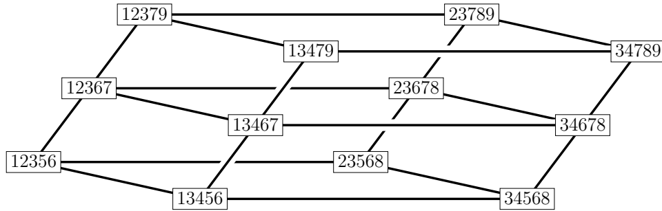
FIGURE 3. The flip graph \mathcal{G}(\bar{\mathbb{Q}}, \bar{\rho}) . Facets of \mathcal{SC}(\bar{\mathbb{Q}}, \bar{\rho}) appear in lexicographic order from left to right.
