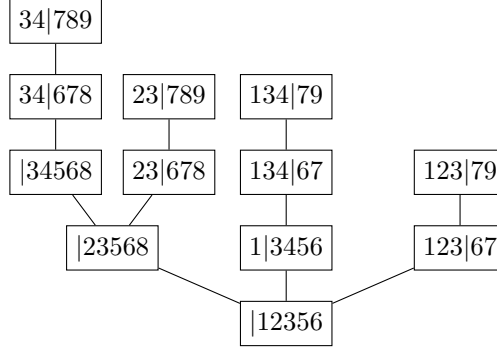
FIGURE 6. The positive greedy flip tree \mathcal{P}(\bar{Q}, \bar{\rho}) on the subword complex of Example 2.2. Each facet I is denoted as the concatenation of its elements. The symbol | separates the elements strictly smaller than \mathfrak{p}(I) from those which are larger or equal to \mathfrak{p}(I) .
