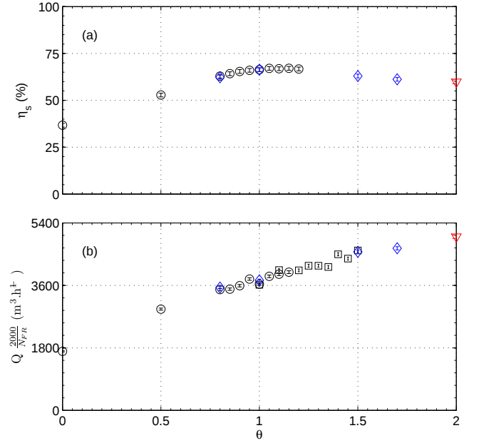
FIG. 11. Maximal static efficiency \eta_s (a) and corresponding nominal flow-rate Q (b) vs \theta for the CRS with S = 10 mm. Black \circ : N_{FR} = 2000 rpm, blue \diamond : N_{FR} = 1600 rpm and red \nabla : N_{FR} = 1300 rpm. Please note that the presented nominal flow-rate has been scaled by 2000/N_{FR}
