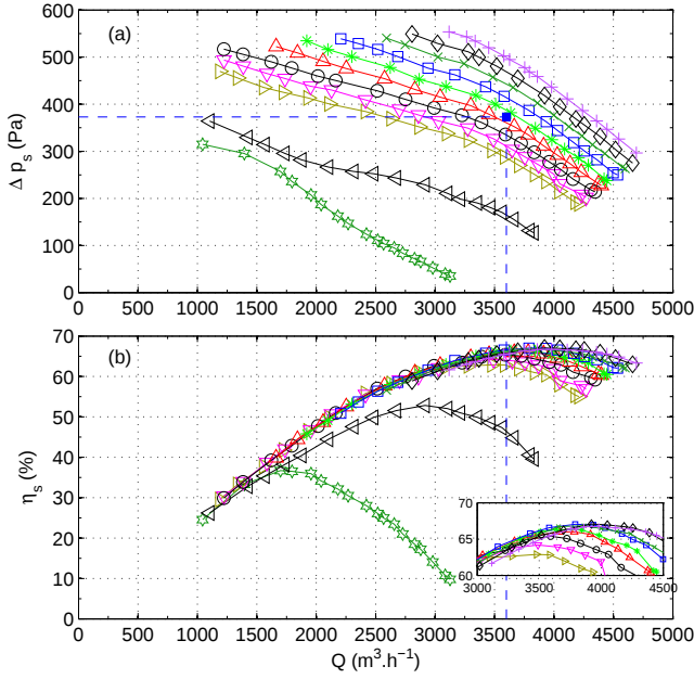
FIG. 10. CRS characteristics at N_{FR} = 2000 rpm, S = 10 mm and \theta \in [0; 1.2] : (a) static pressure rise \Delta p_s vs flow rate Q ; (b) static efficiency \eta_s vs flow rate Q . Dark green \star : \theta = 0 , black \triangleleft : \theta = 0.5 , mustard yellow \triangleright : \theta = 0.8 , magenta \nabla : \theta = 0.85 , black \circ : \theta = 0.9 , red \triangle : \theta = 0.95 , green * : \theta = 1 , blue \square : \theta = 1.05 , dark green \times : \theta = 1.1 , black \diamond : \theta = 1.15 and purple + : \theta = 1.2 . The blue \blacksquare and the dashed lines stand for the design point of the CRS
