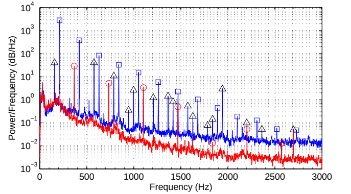
FIG. 7. Power spectral density of the wall pressure fluctuations 5 mm downstream the front rotor. The blue curve stands for the axial spacing S = 10 mm and the red curve for S = 150 mm. The red \circ stand for the blade passing frequency and the harmonics of the front rotor and the blue \square stand for that of the rear rotor. The black \triangle stand for the various interactions of these frequencies
