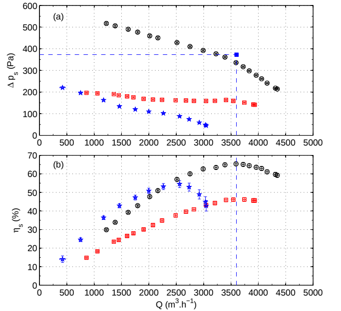
FIG. 3. Fans characteristics: (a) static pressure rise \Delta p_s vs flow rate Q ; (b) static efficiency \eta_s vs flow rate Q . The axial spacing is S = 10 \text{ mm} . Red \square : FR rotating alone at N_{FR} = 2000 rpm (RR has been removed), blue \star : RR rotating alone at N_{RR} = 1800 rpm (FR has been removed) and black \circ : CRS at N_{FR} = 2000 rpm and \theta = 0.9 . The blue \blacksquare and the dashed lines stand for the design point of the CRS. The errorbars stand for the measurement uncertainty
