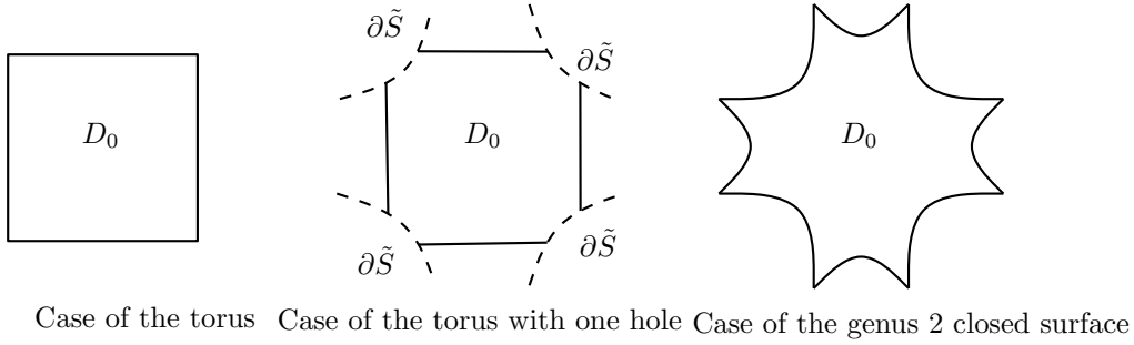
Figure 1: The fundamental domain D_0
