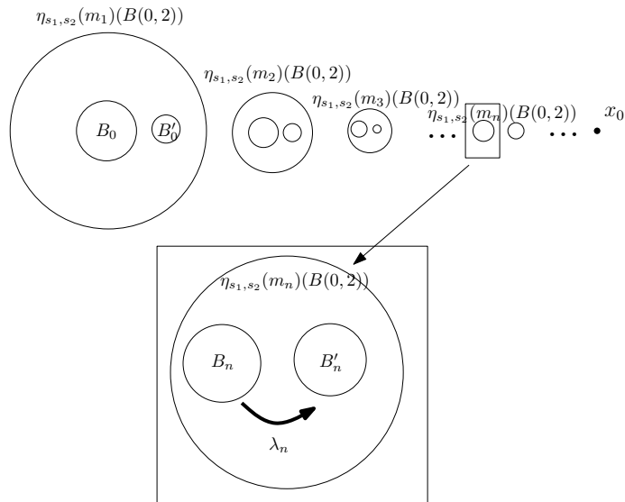
Figure 4: Notations in the proof of lemma 4.4
